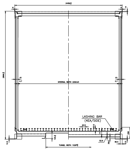
SECTION C-C (ROTATED 90°) SCALE 1:25
